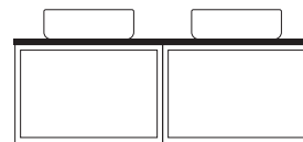
120cm Wall Hung Double Unit 1200(w) x 402(h) x 455(d)mm (Excl. Basin) Two soft close drawers
